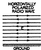
Horizontal polarization.
